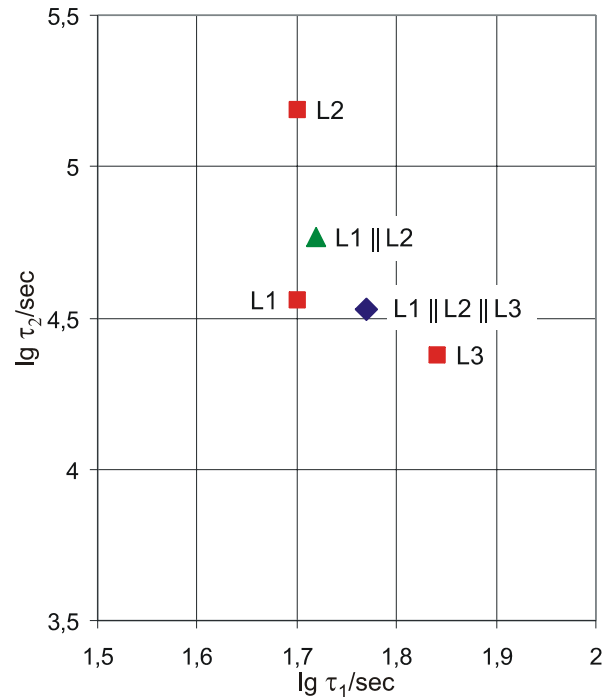
Fig. 5: Dielectric time constants \tau_1 and \tau_2 for the measurements with 62 \text{ G}\Omega (selection from Table 1).
