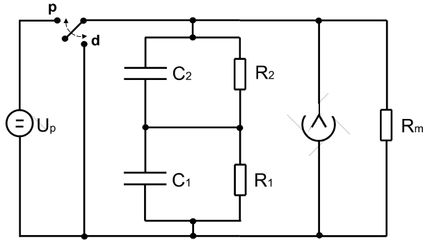
Fig. 2: Equivalent circuit of a paper-oil-dielectric with \tau_2 = R_2 C_2 and \tau_1 = R_1 C_1 and basic measuring circuit
