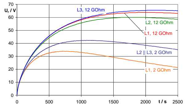
Fig. 4: Return voltage curves from measurements of the three cores L1, L2 and L3 of a 1300 m long cable (TOR) with different measuring resistors
