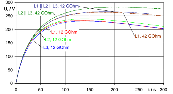
Fig. 3: Return voltage curves from measurements of the three cores L1, L2 and L3 of a 150 m long cable (GA9) with different measuring resistors
