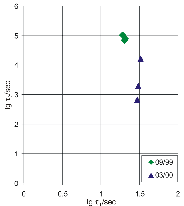
Fig. 7: Change of the dielectric time constants as a consequence of ageing during 6 months (see table 3)
