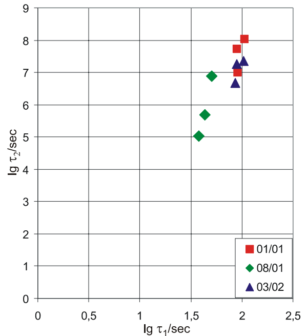
Fig. 6: Dielectric time constants for measurements of cable DYR in different seasons of the year (see table 2)
